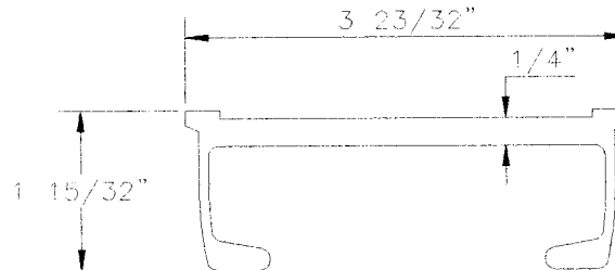
TYPE 35-4 LRNS DECK SLAT 1.578 LBS. PER FT. PART NO. 41-3157
