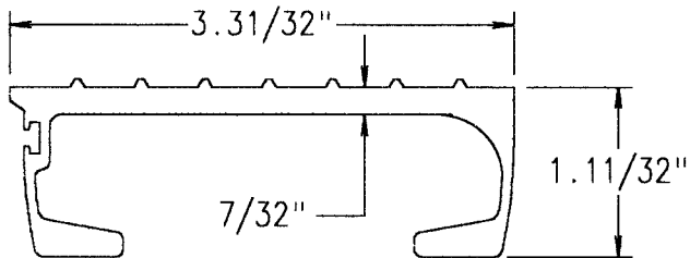
Type 40-3.5 Deck Slat Part No.: 41-2951 1.726 lbs. per ft.
