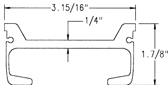
Type 40-4 Double Ridge Part No. 41-3795 2.294 lbs. per ft.
