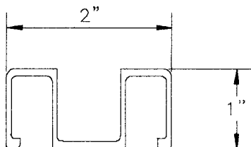
ALUMINUM SUBDECK .51 LBS. PER FT. PART NO. 41-2460
