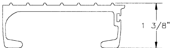
TYPE 35-3 DECK SLAT 1.415 LBS. PER FT. PART NO. 41-275
