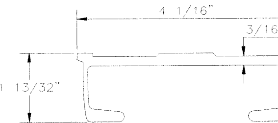
TYPE 40-3 LRNS DECK SLAT 1.675 LBS. PER FT. PART NO. 41-3086
