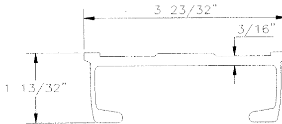
TYPE 35-3 LRNS DECK SLAT 1.445 LBS. PER FT. PART NO. 41-3075
