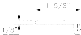
ALUMINUM SIDE TRIM NO SEAL .322 LBS. PER FT. PART NO. 41-166NS
