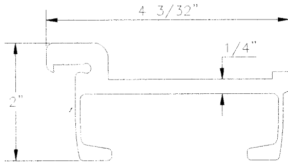
TYPE 35-4 NLR DECKSLAT 2.209 LBS. PER FT. PART NO. 41-3281
