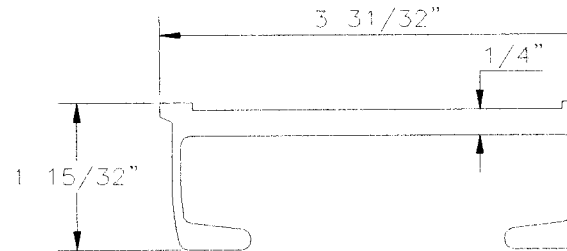
TYPE 37-4 LRNS DECK SLAT 1.754 LBS. PER FT. PART NO. 41-3082
